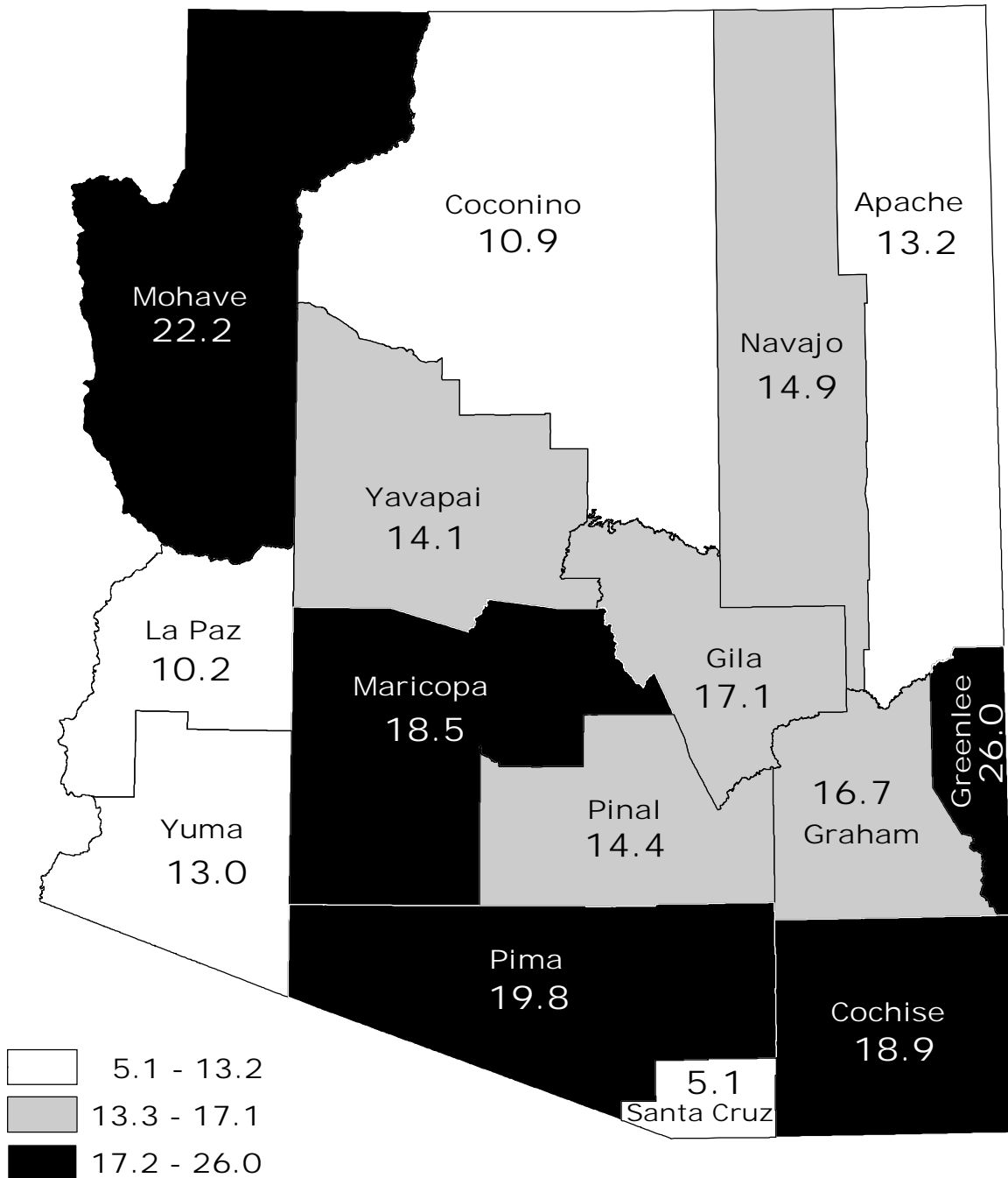
Figure 7B-9 Mortality from Colorectal Cancer by County of Residence, Arizona, 2003
