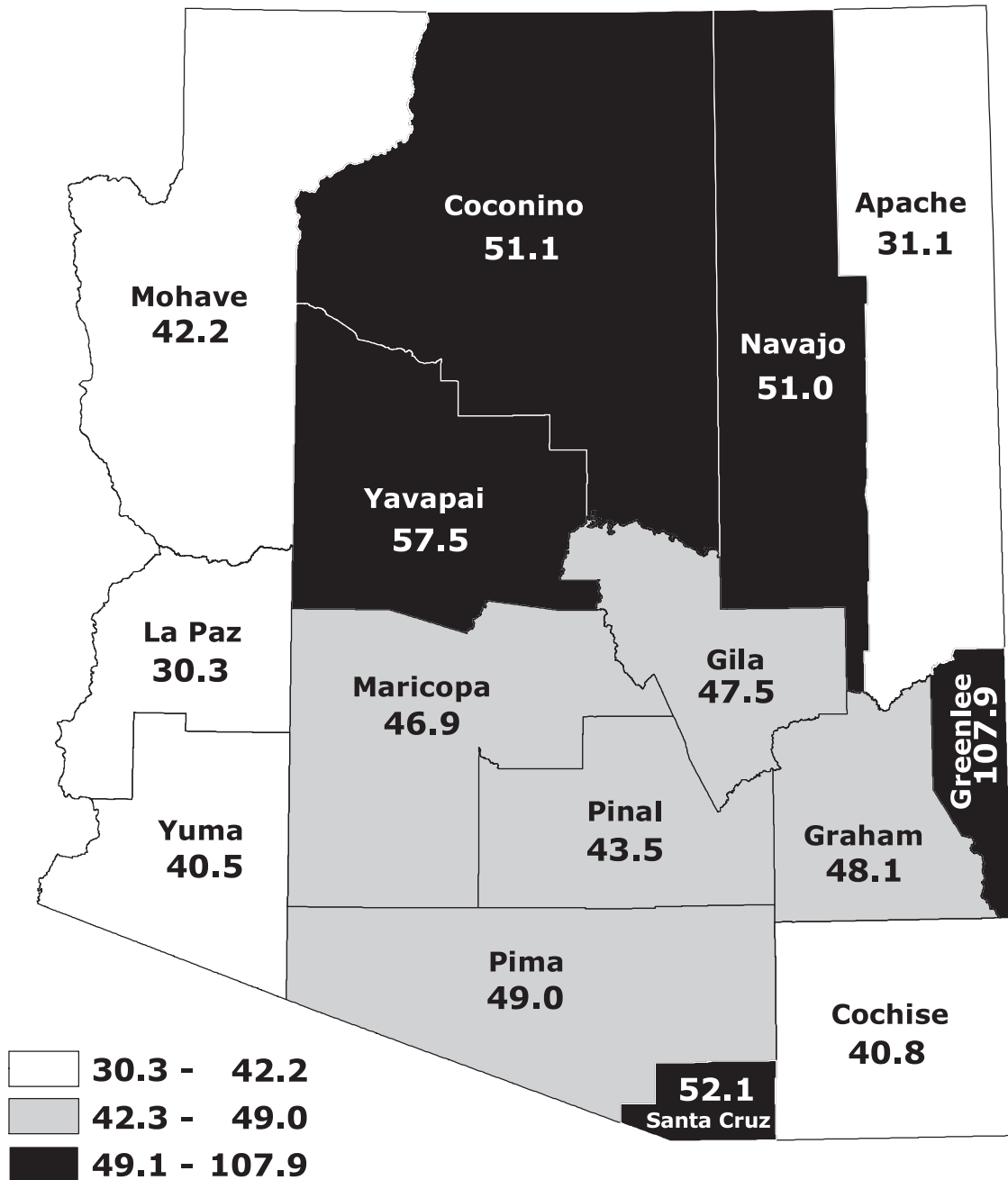
Figure 7B-4 Mortality from Cerebrovascular Disease by County of Residence, Arizona, 2002
